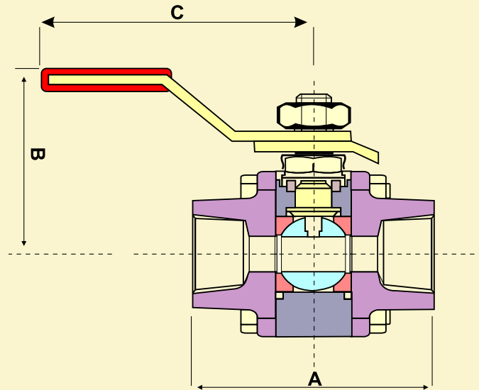
SCREWED END
