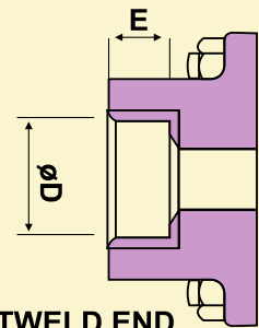
SOCKETWELD END
